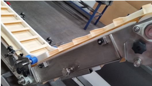
Remove Side Guides
